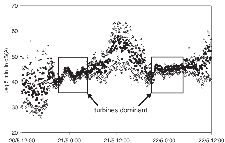
Fig. 4. 48 h registration of immission level ( L_5 = \triangle ; L_{eq} = \bullet ; L_{95} = \circ ) per 5 min at location A; turbines are considered the dominant sound source if L_5 - L_{95} \leq 4 dB.
